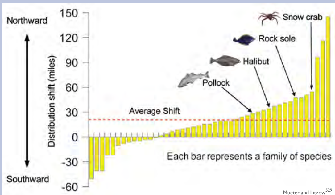
Marine Species Shifting Northward 1982 to 2006
