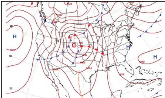
Sea Level Pressure and Frontal Systems
